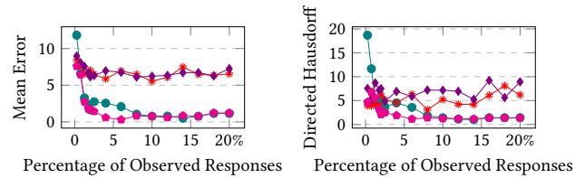
Figure 12: Mean Error and DH for Grid Database(20x20) under a uniform query distribution (Tamassia et al. [64, 66] (—●—), Kamada Kawai [38] (—■—), Chrobak & Payne [12] (—◆—), Fruchterman Reingold [25] (—*—)).
