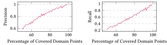
Figure 10: We use the Grid(25x25) dataset to show the effectiveness of our attack. We randomly remove records from the Grid database (horizontal axis) and measure the precision, and recall of Algorithm 5 on these databases of different density. The adversary observes 20% (uniformly at random) of the responses on all runs.
