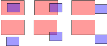
Figure 2: We see that no matter how the rectangles overlap, their intersection forms a rectangle, potentially of lower dimension (i.e., a line segment or a point).
