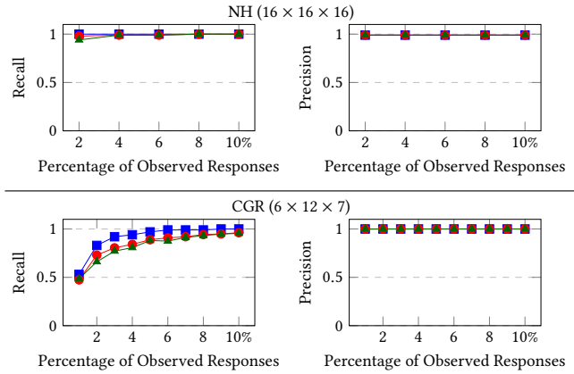
Figure 9: Recall and precision of our attack on the 3D datasets as a function of the percentage of all responses observed by the adversary under three query distributions (Uniform (—■—), Beta(2,1) (—●—), Gaussian (—▲—)).
