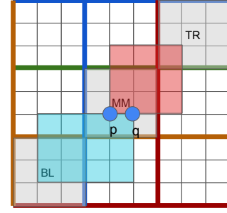
Figure 6: (A 2D example) Algorithm 5 reconstructs the \lambda -core of the database ( MM ) after observing O\left(\frac{2^d}{(1 - \sqrt[d]{\lambda})^d} m \log m\right) queries uniformly at random. We show that for each pair p, q , with high probability, we observe a blue response, which starts at BL and ends at q , and a red response, which starts at p and ends at TR . The intersection of the two, gives us a response that contains only the neighbors p, q .
